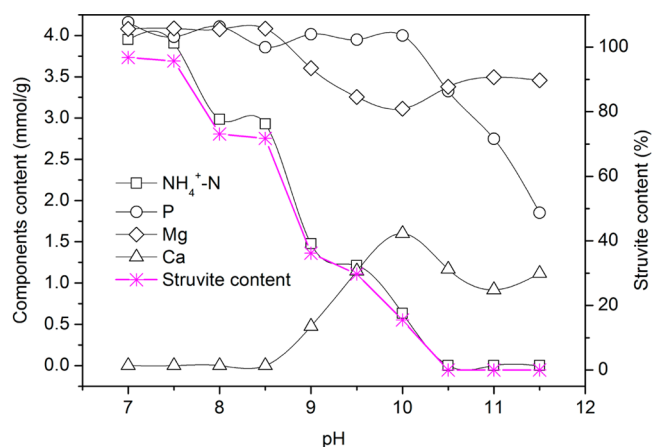
Figure 1. Elemental analyses of the precipitates from synthesized wastewater at different pHs 4 (Components content: element molar (mmol)/weight of the precipitates (g)).
